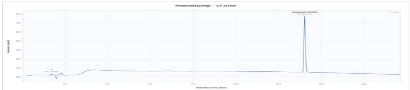
Retatrutide 10mg - Batch26-0616A: UV Chromatogram
