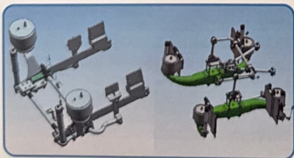
New design suspension system enhancing stability, comfort and safety.
