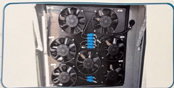
Intelligent ICS cooling system with SPAL brushless electric fan.
